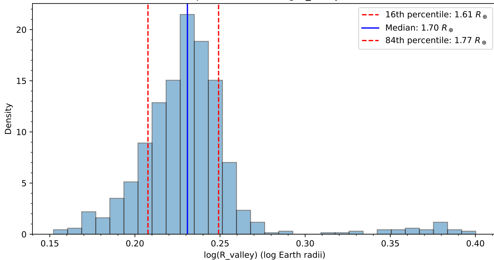
Bootstrap Distribution of \log(R_{\text{valley}}) , bin 4
